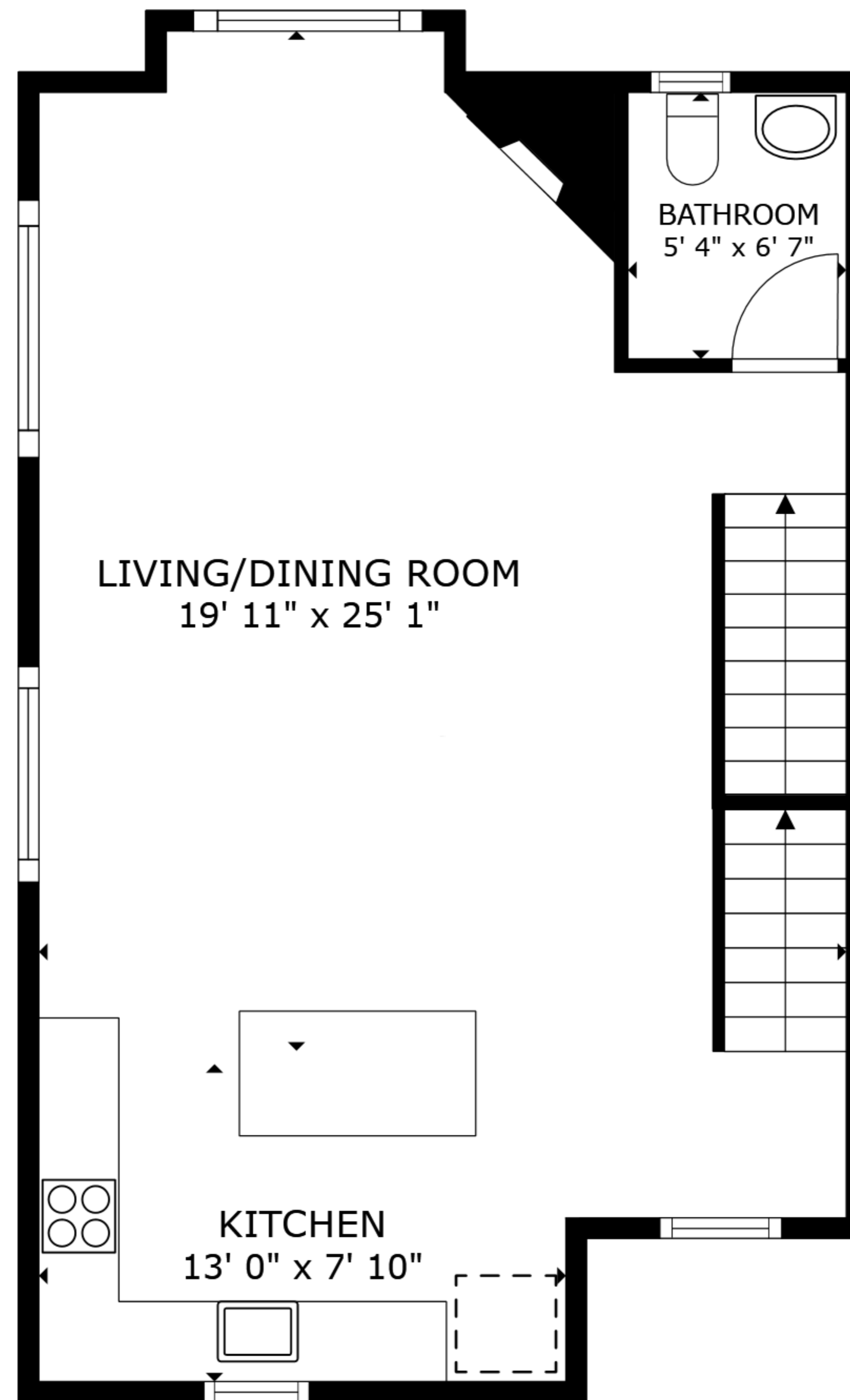
FLOOR 2
